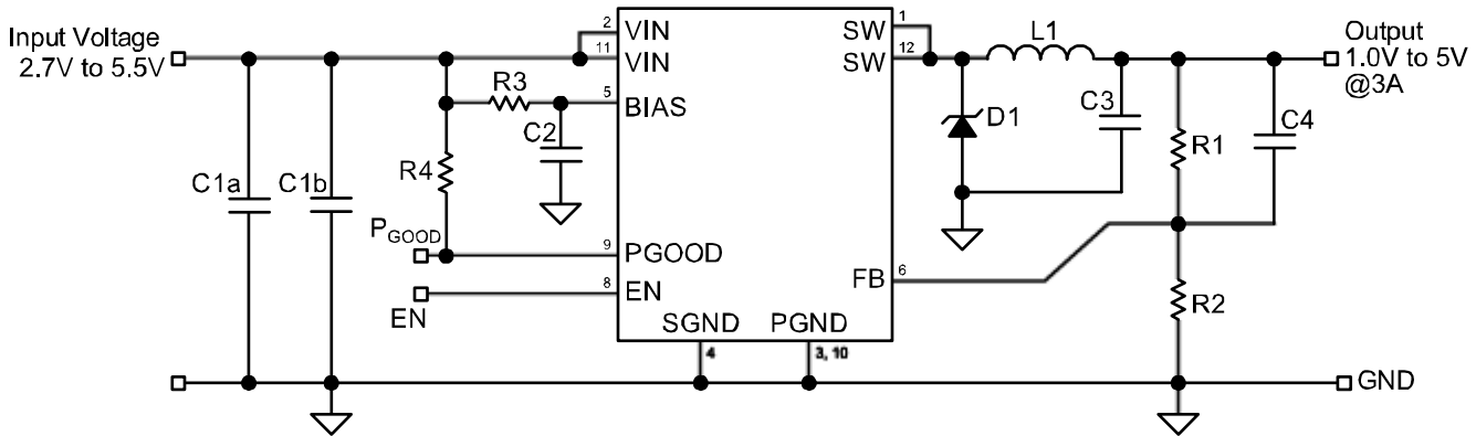
MIC2207 Schematic
